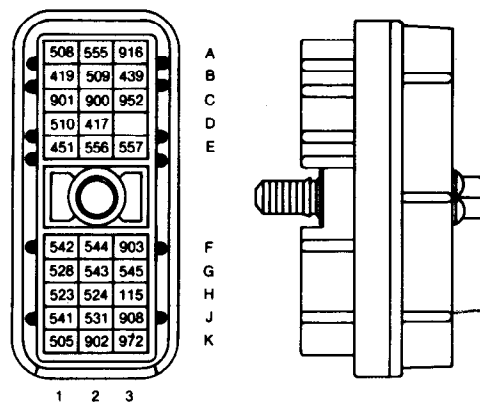
ECM Vehicle Harness Connector P/N 12034398
