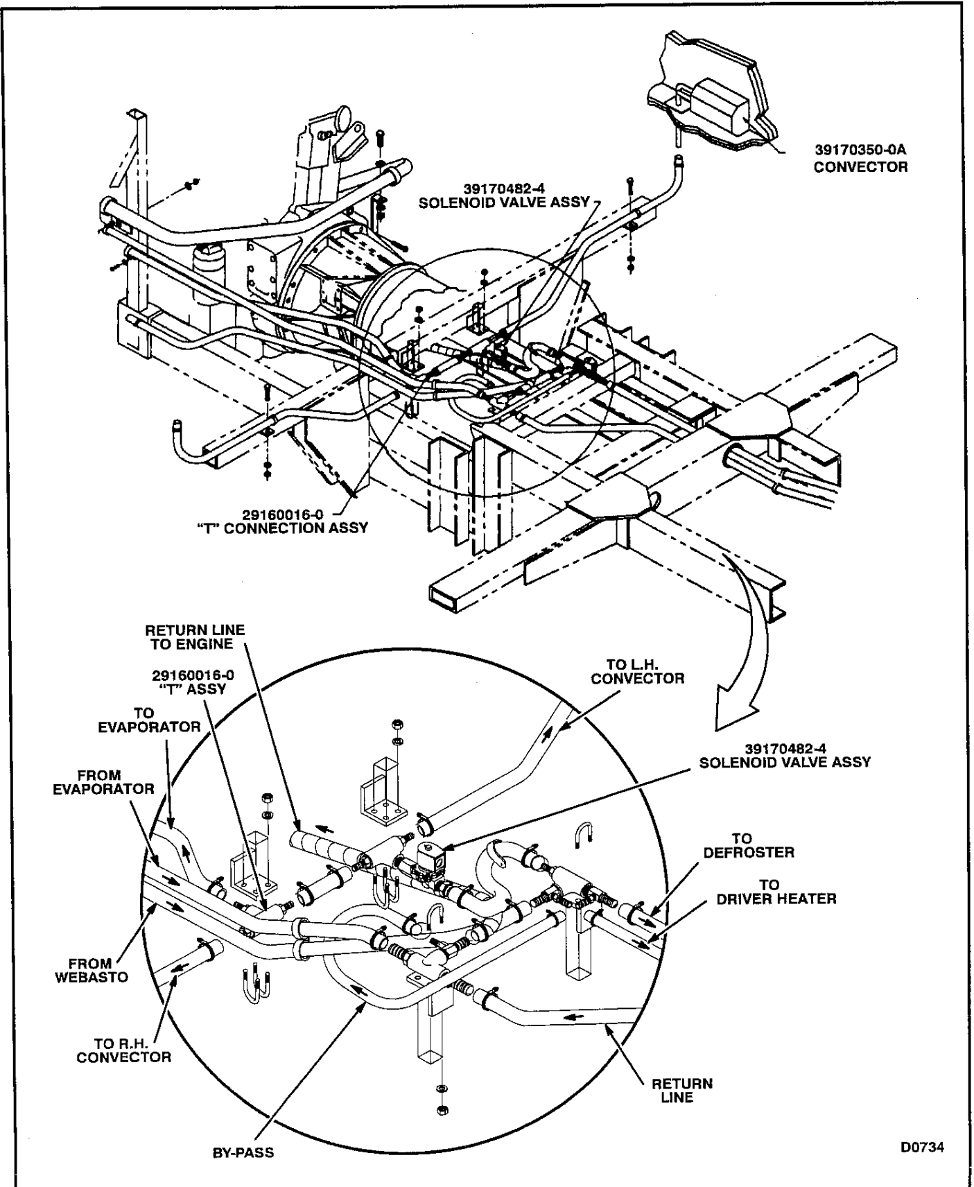
Figure 2. Existing Heating System Piping at Rear of Coach.
