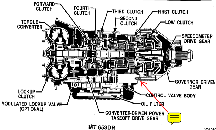
Transmission Cross-Section Showing Internal Components
